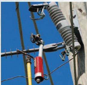
FT-1 being used to remove a blown fuse
