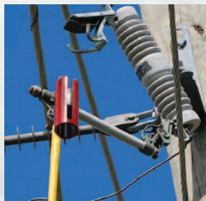
FT-1 being used to close in a new fuse
